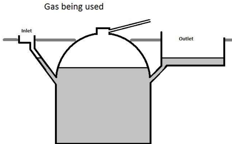
Figure 3 Maximum Pressure - gas should be burned off before this point!
