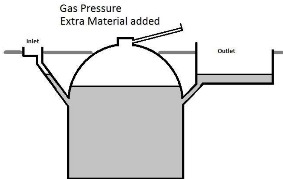
Figure 2 Filling and Biogas Generation
